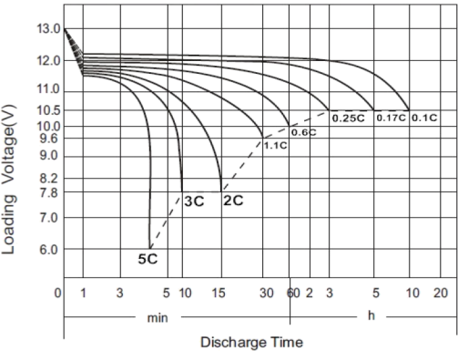
Discharge Characteristics
