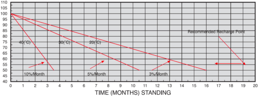
Discharge Characteristics
